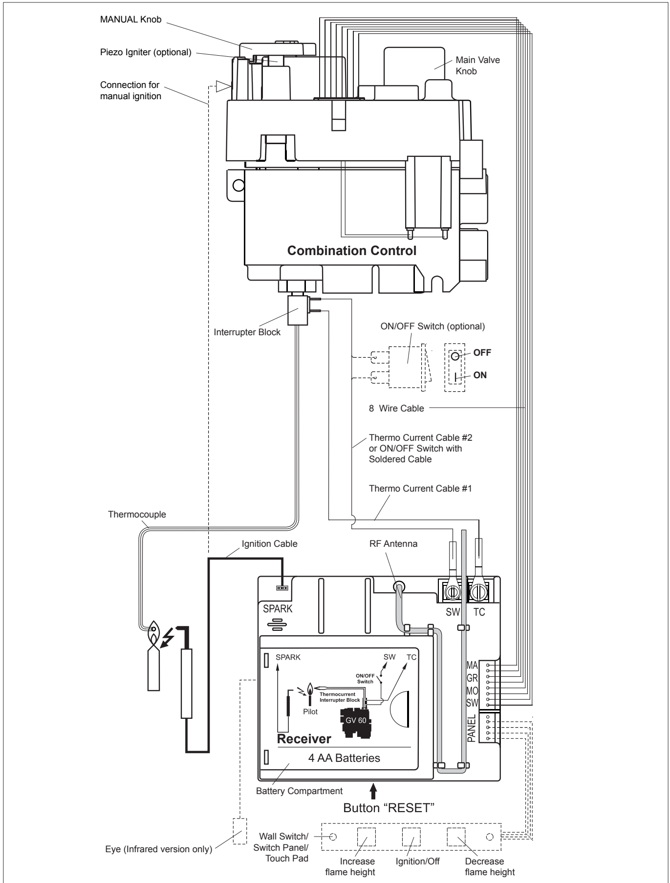
Figure 17: Wiring Diagram
